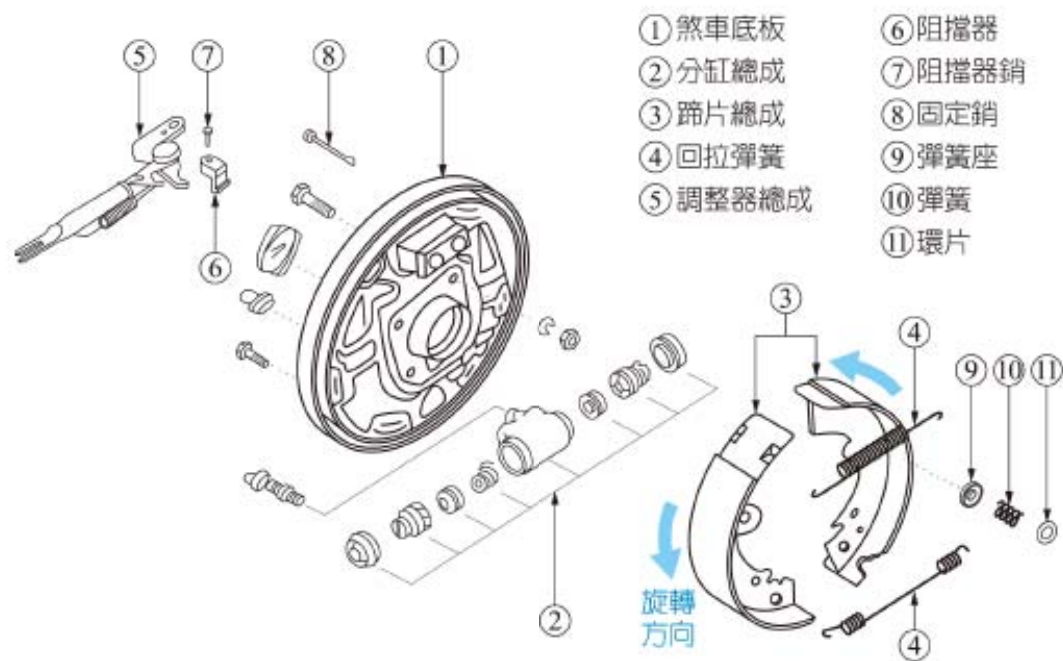
(C)分解圖
